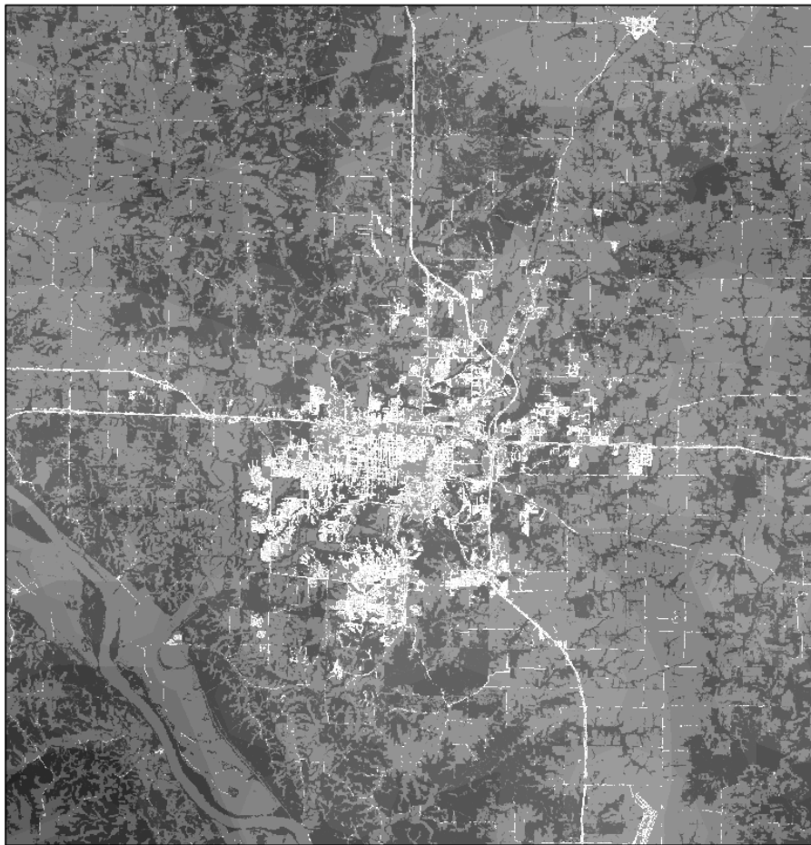
Figure 4: Preliminary Output of ArcGIS showing favorable locations for level spreaders (white and light gray areas)
