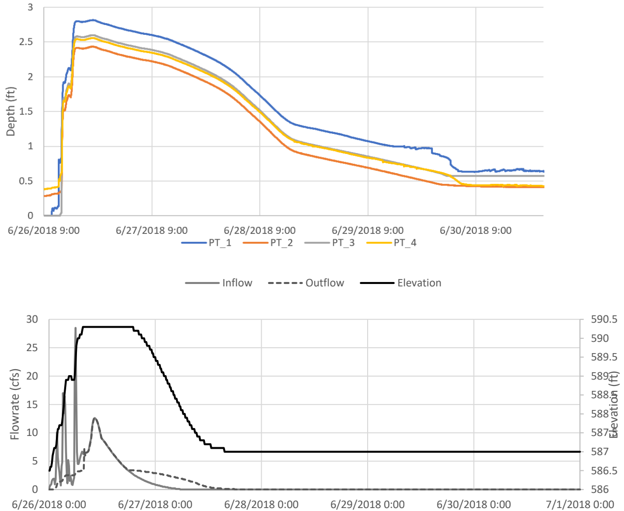
Figure 3: HEC-HMS and Pressure transducer results for water elevation and depth over a 5-day period during and after rain event
