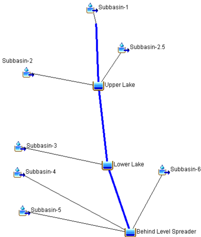
Figure 2: HEC-HMS Basin framework used to model the level spreader watershed
